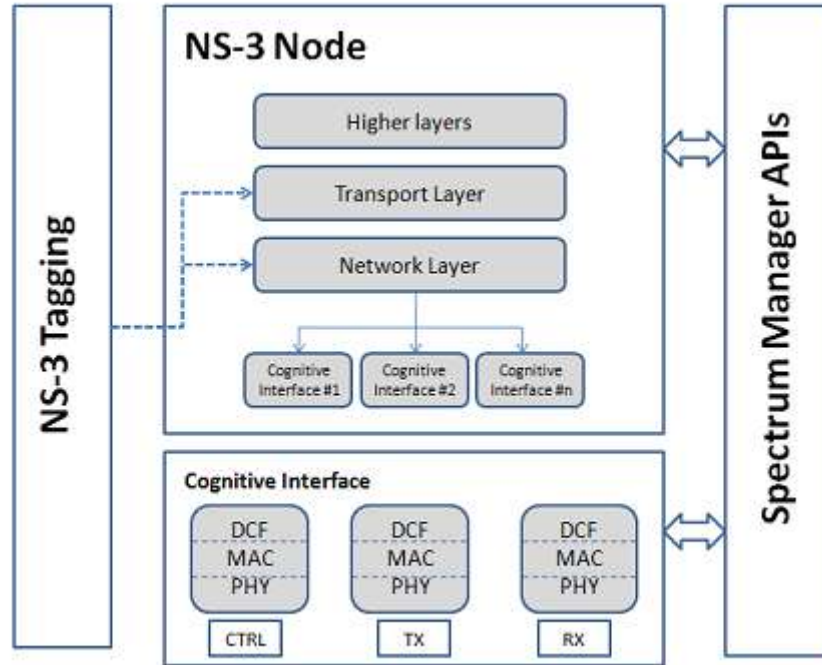
Figure 2: Layered Architecture of an NS-3 CR Node
